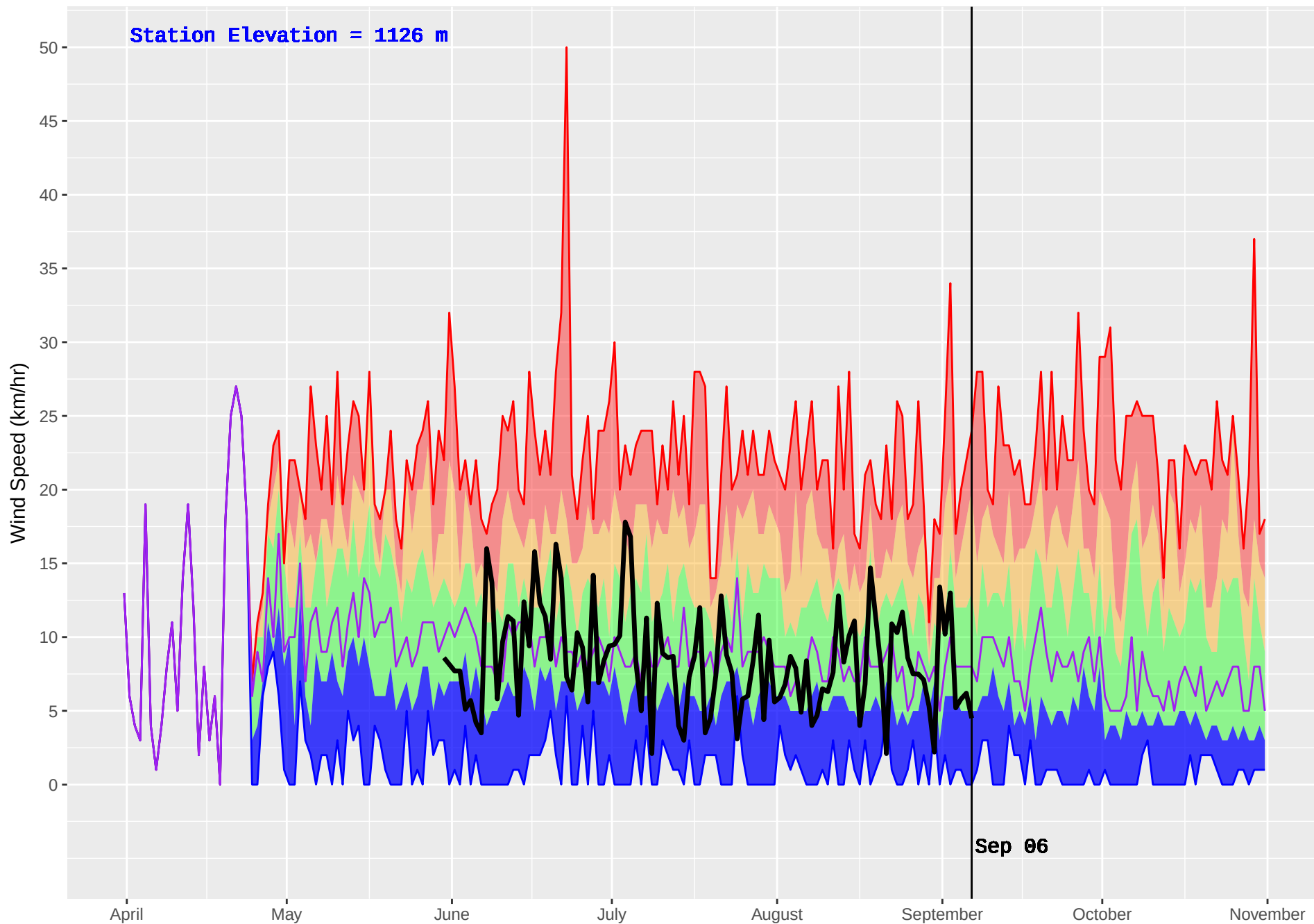
BLACKPINE (148) : Historical (1980–2016) and Current (2017) Noon Wind Speed
