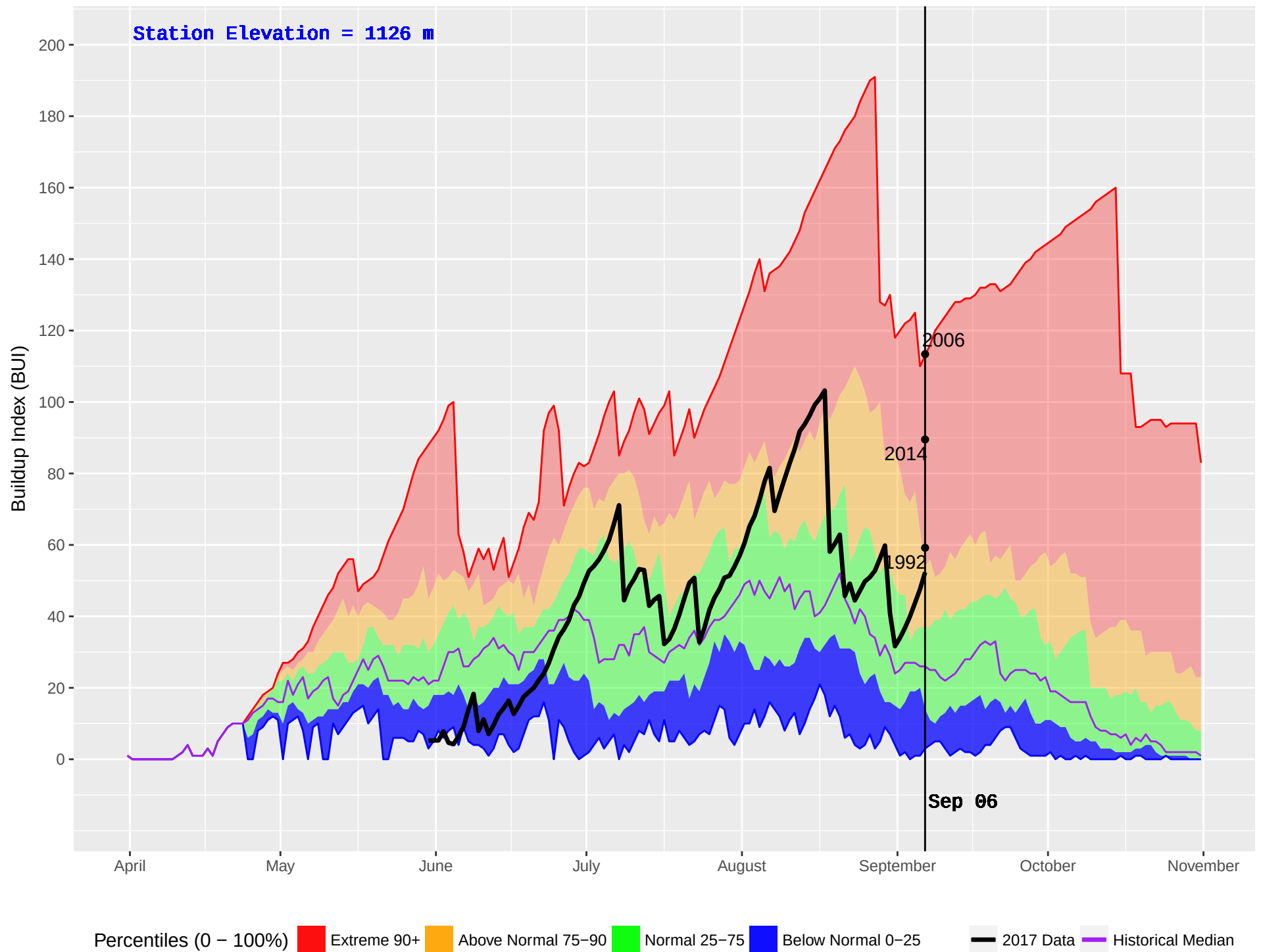
BLACKPINE (148) : Historical (1980–2016) and Current (2017) Noon Buildup Index (BUI)
