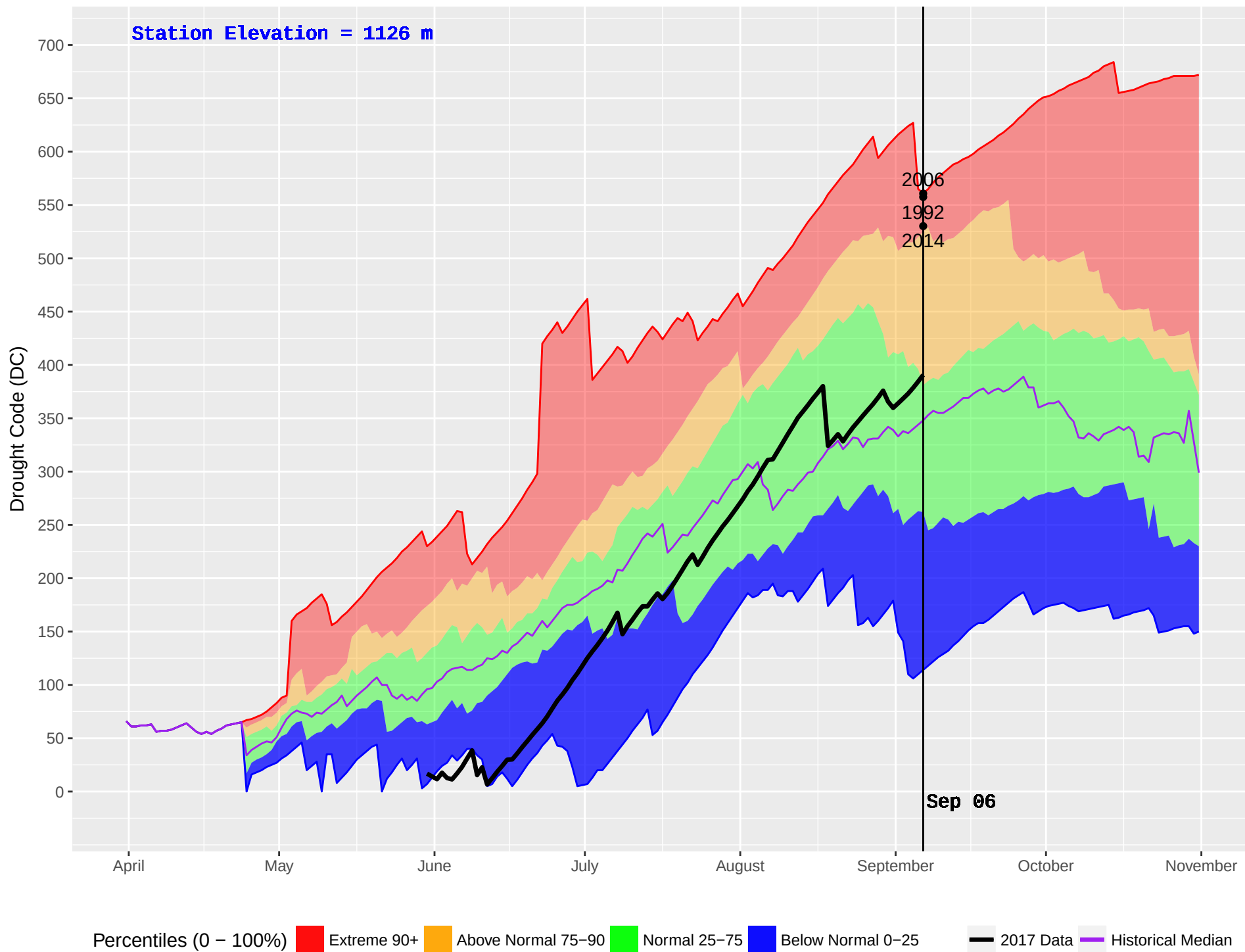
BLACKPINE (148) : Historical (1980–2016) and Current (2017) Noon Drought Code (DC)
