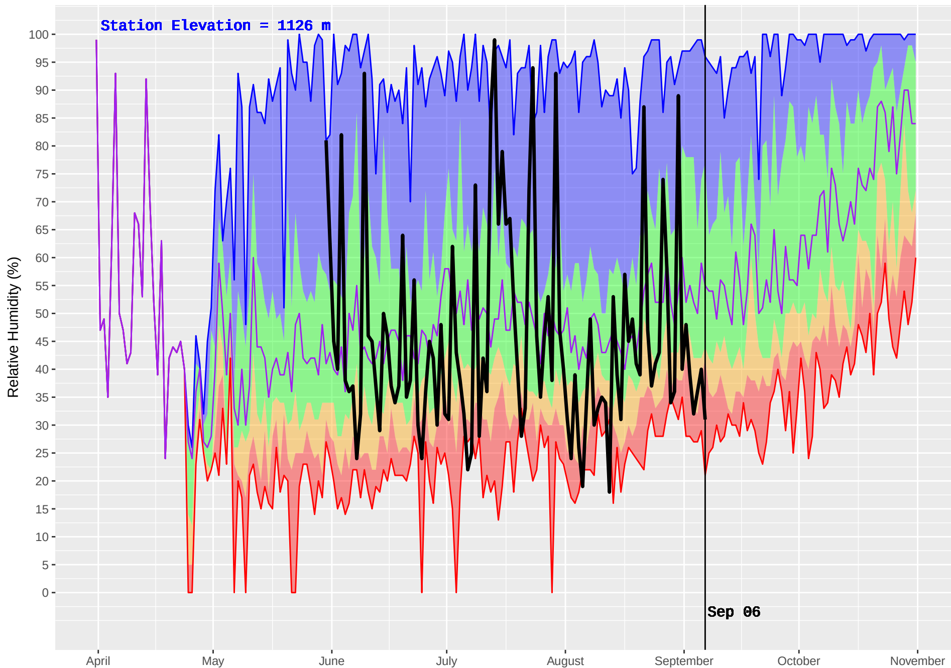
BLACKPINE (148) : Historical (1980–2016) and Current (2017) Noon Relative Humidity
