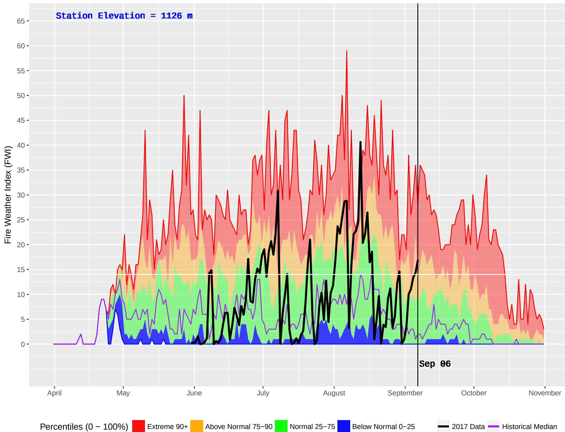
BLACKPINE (148) : Historical (1980–2016) and Current (2017) Noon Fire Weather Index (FWI)
